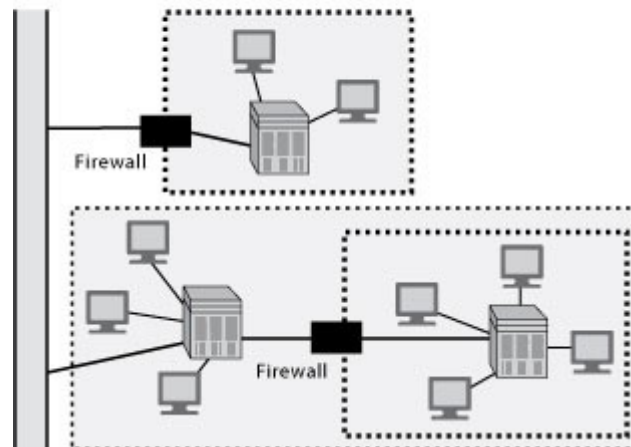
Fig. 2.4: An extranet
