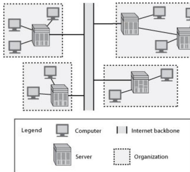
Fig. 2.2: The Internet
