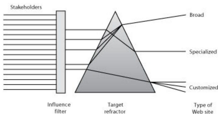
Fig. 3.3: Attractor strategies
