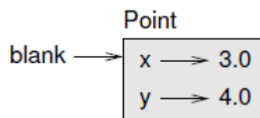
Fig. 15.1: Figure 15.1: Object diagram.
