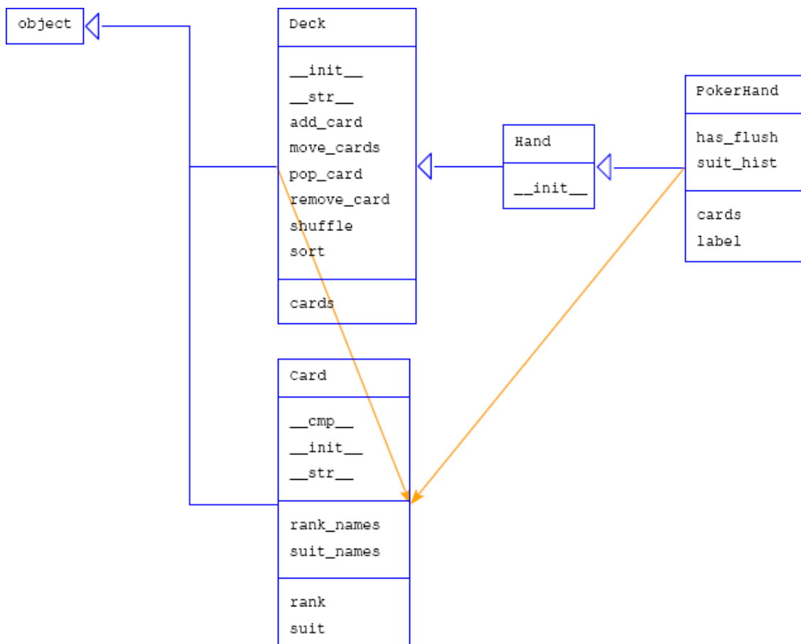
Fig. 19.10: Figure C.8: Class diagram.
