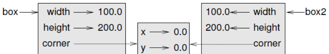
Fig. 15.3: Figure 15.3: Object diagram.
