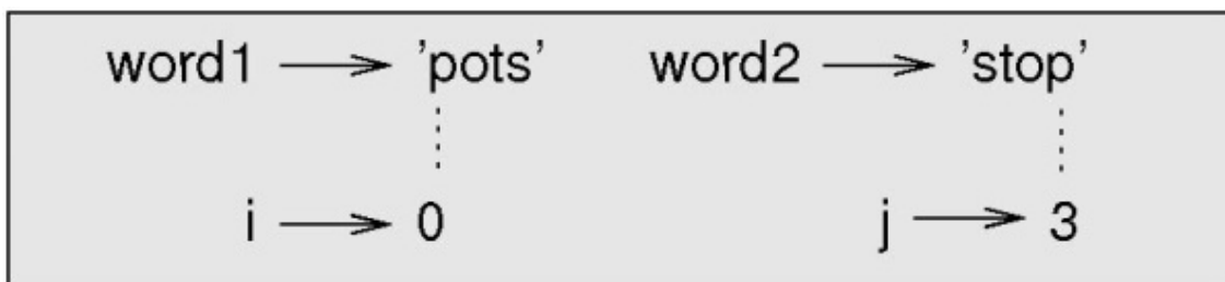
Fig. 8.2: State diagram.
