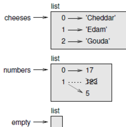
Fig. 10.1: State diagram
