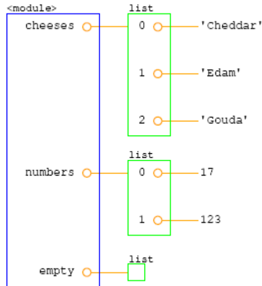
Fig. 19.5: Figure C.3: Object diagram.
