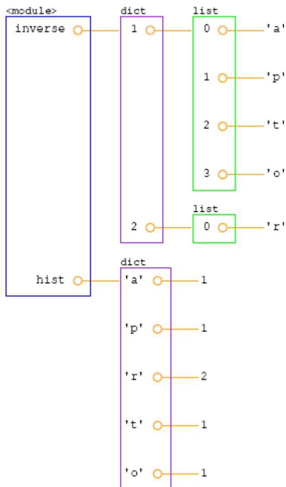
Fig. 19.6: Figure C.4: Object diagram.
