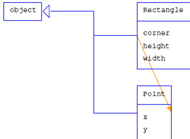
Fig. 19.9: Figure C.7: Class diagram.
