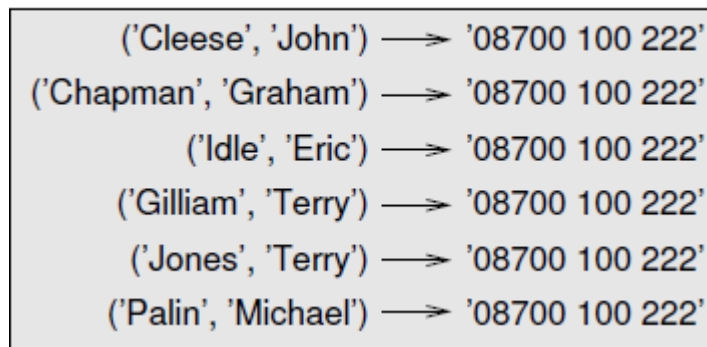
Fig. 12.2: Figure 12.2: State diagram.
