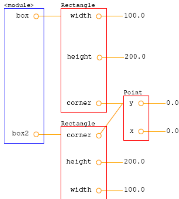
Fig. 19.7: Figure C.5: Object diagram.
