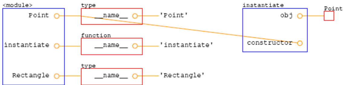
Fig. 19.8: Figure C.6: Object diagram.
