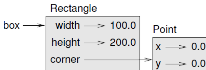
Fig. 15.2: Figure 15.2: Object diagram.
