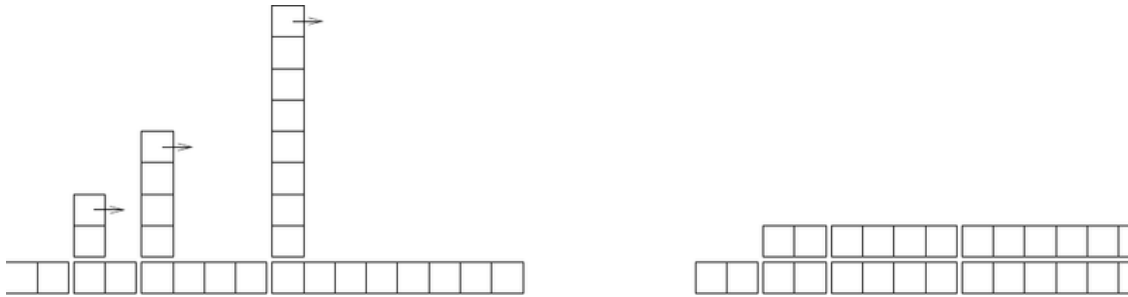
Fig. 19.2: Figure B.1: The cost of a hashtable add.
