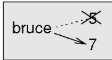
Fig. 7.1: State diagram.
