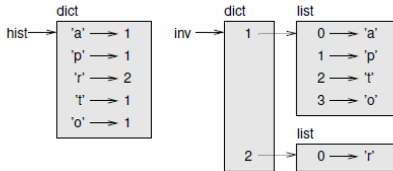
Fig. 11.1: State diagram
