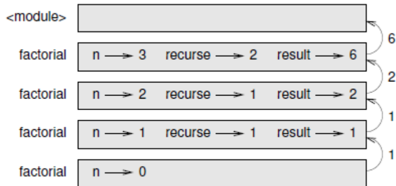
Fig. 6.1: Stack diagram
