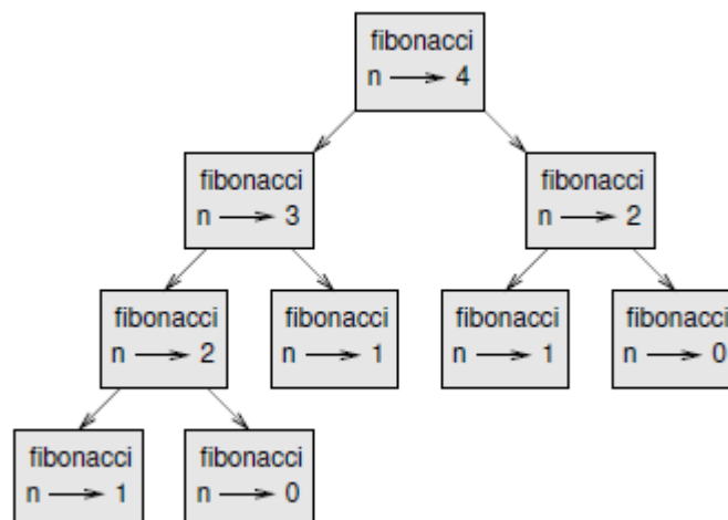
Fig. 11.2: Call graph.
