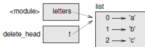
Fig. 10.5: Stack diagram.
