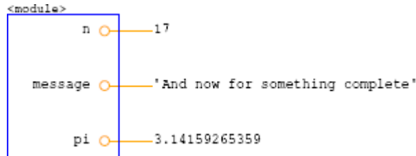
Fig. 19.3: Figure C.1: State diagram generated by Lumpy.
