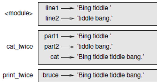
Fig. 3.1: Stack diagram.
