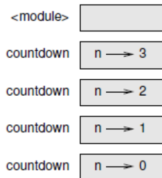
Fig. 5.1: Stack diagram
