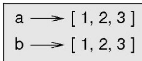
Fig. 10.3: State diagram.
