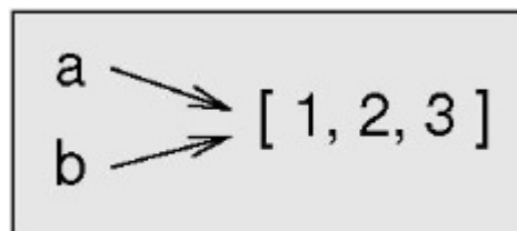
Fig. 10.4: State diagram
