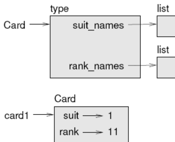
Fig. 18.1: Figure 18.1: Object diagram.
